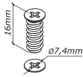
V114 x5
